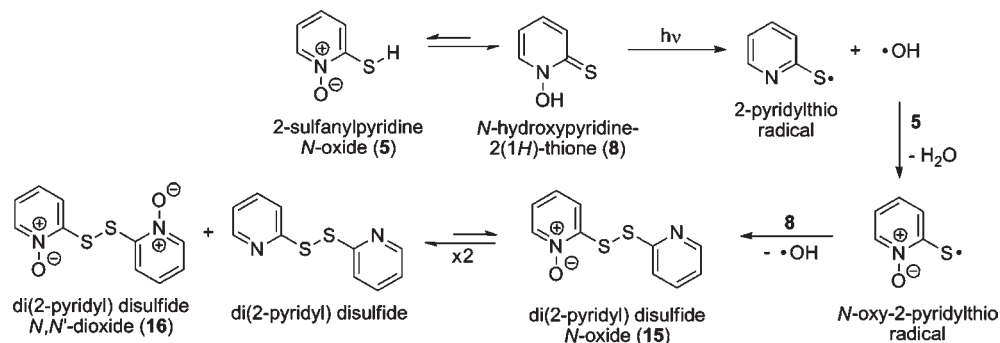
Figure 4. Proposed formation of pyridyl-containing compounds from pyrithione (adapted with permission from ref 20).
